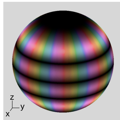
c / A wavefunction on the sphere with |\mathbf{L}| = 11\hbar and L_z = 8\hbar , shown using the color conventions defined in figure u, p. 884.
